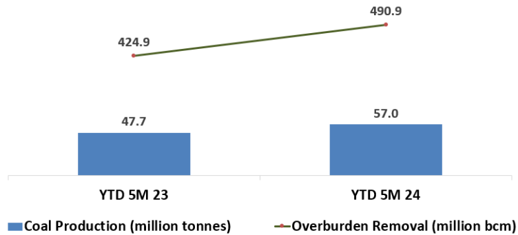
Coal Production and Overburden Removal
